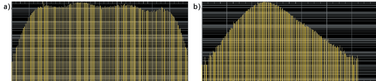
Figure 11. Histograms of jitter measured by the JS-1000. In (a) the DUT has large contributions of DJ; and in (b), the DUT has little DJ.
